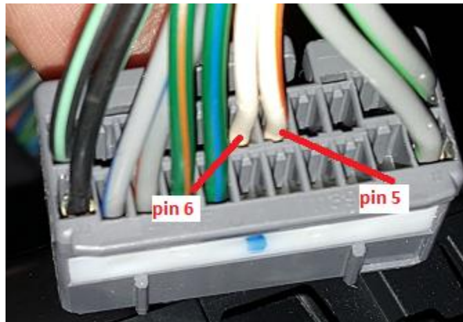
This is the wire view of the connector in the vehicle
